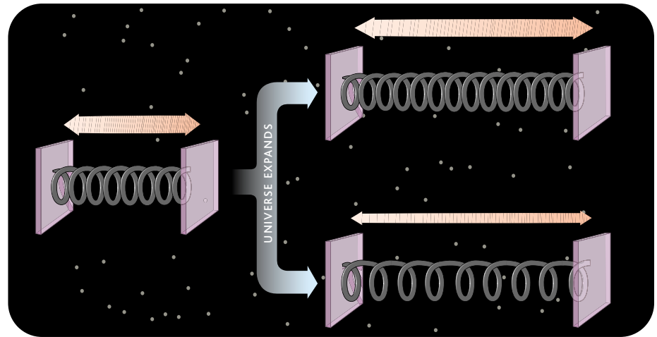
Loaded question. Dark energy acts like a spring that stretches space. If it's a cosmological constant, the spring grows with space to maintain a constant push (top). Otherwise, the push may vary (bottom).
